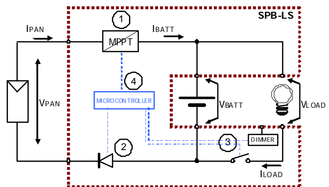
Fig. 2 Principle diagram
